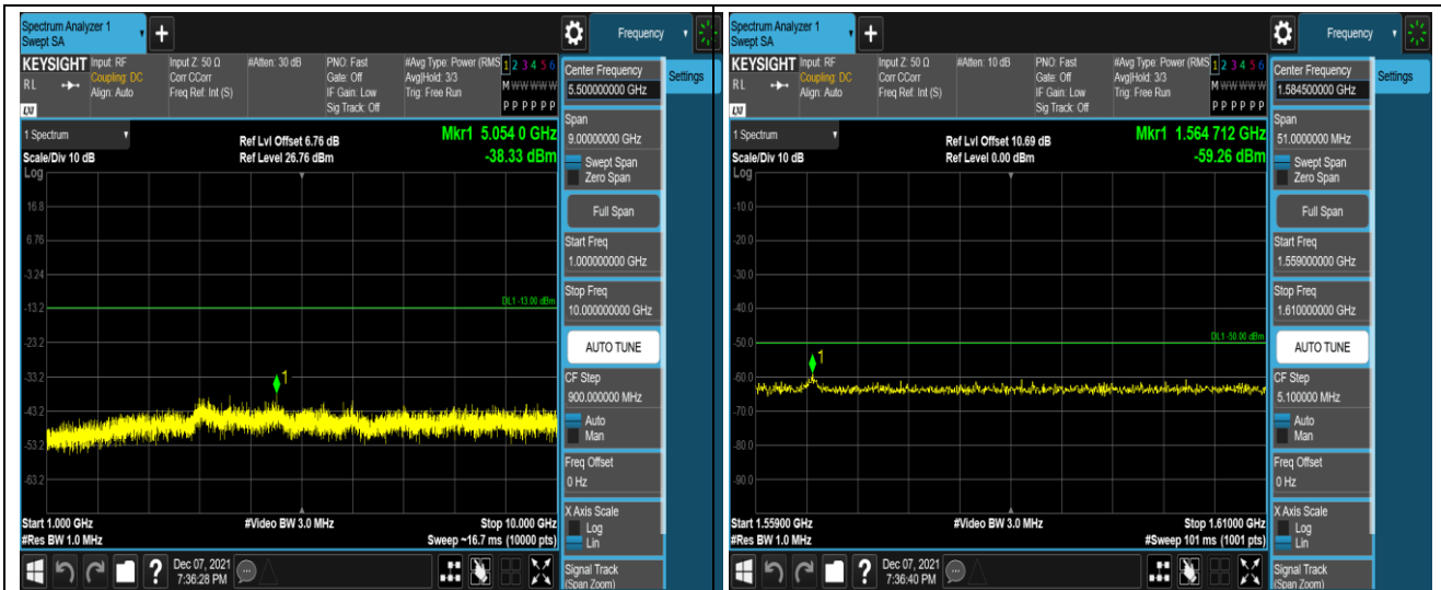
Band13-5MHz-16QAM-23255-1RB#0-Range2:1000~10000MHz
