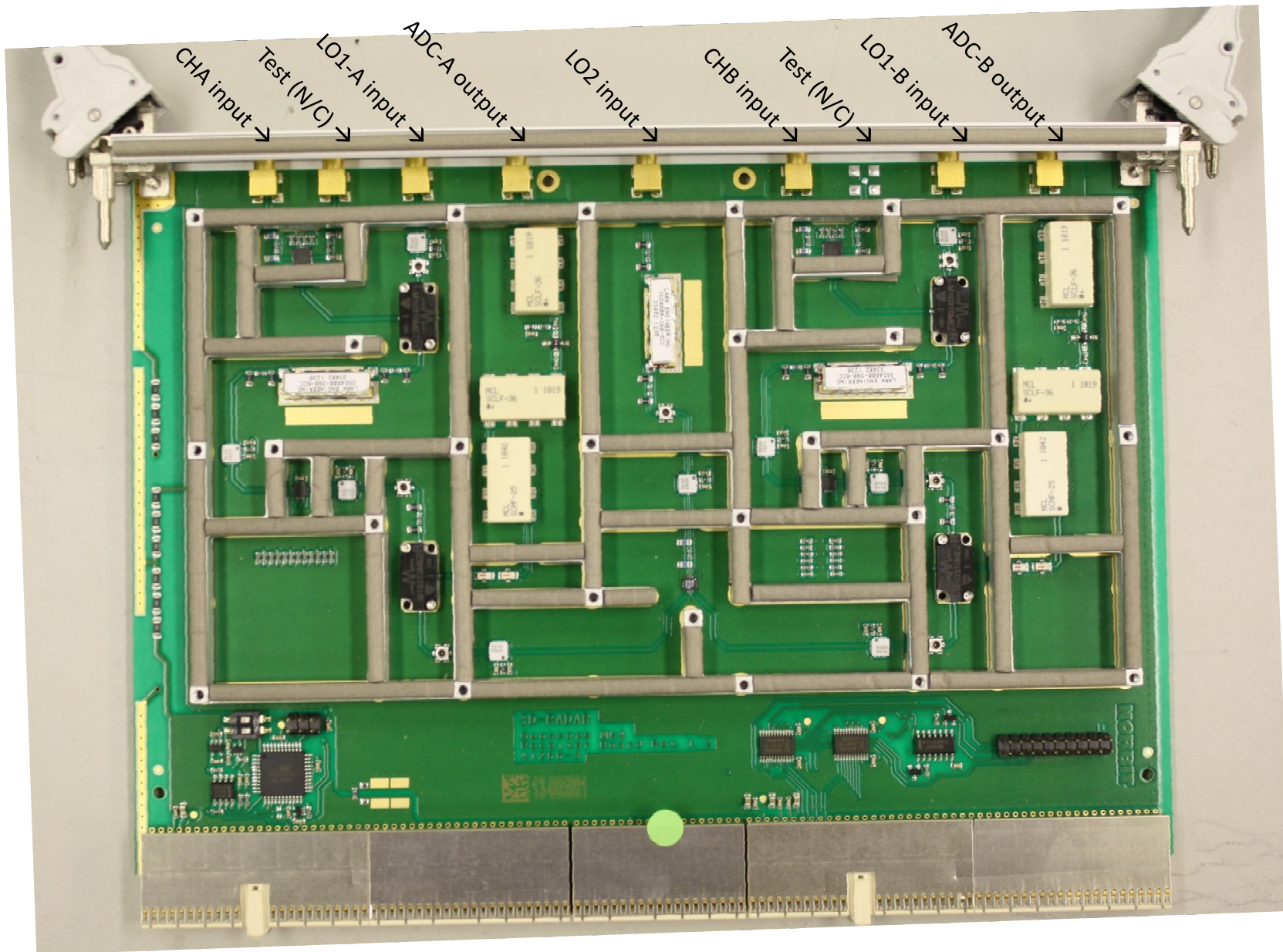
3d-Radar Geoscope Dual-Channel Receiver board. Top view. Shield removed.
