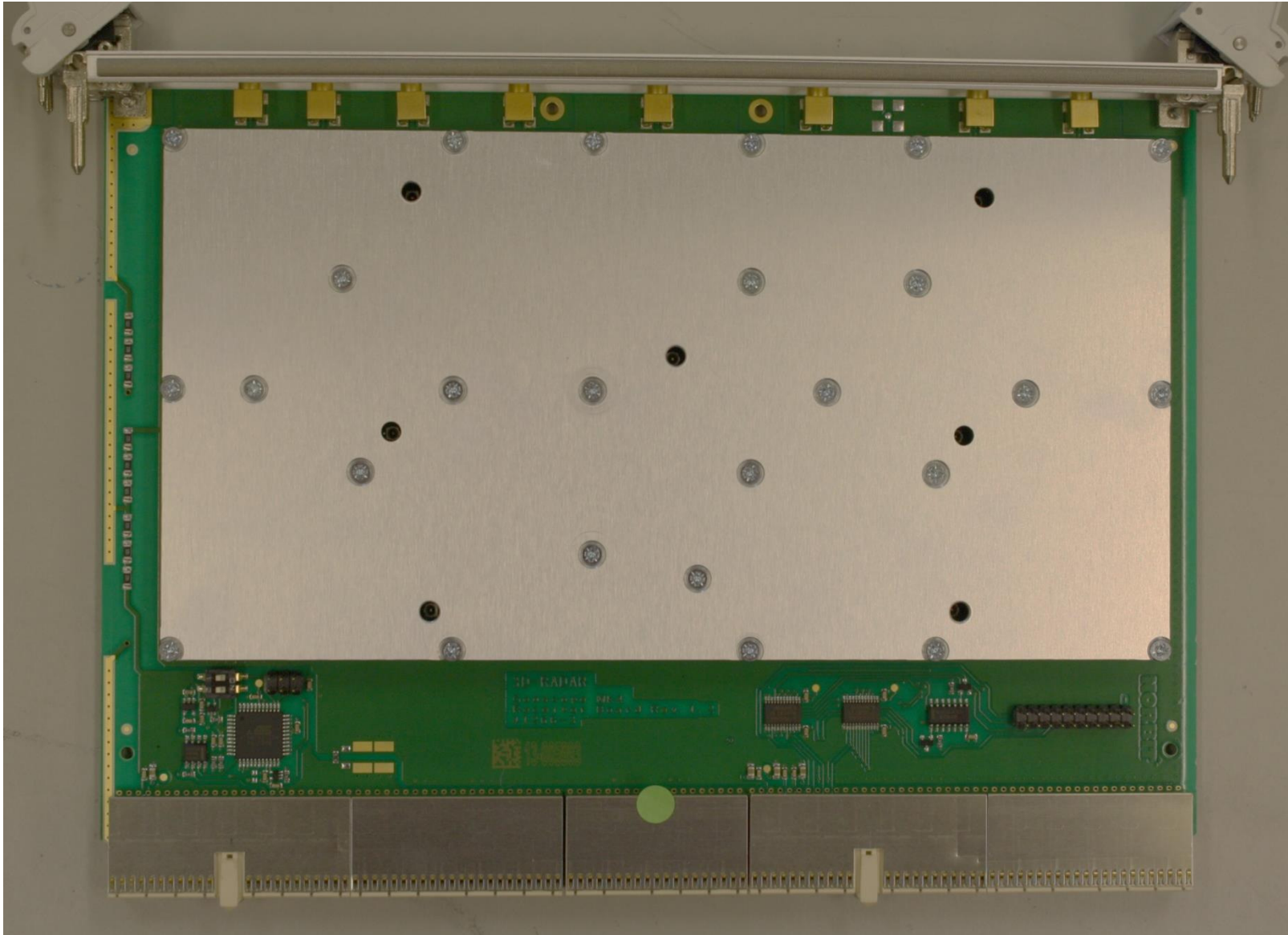
3d-Radar Geoscope Transmitter board. Top view. Shielded.
