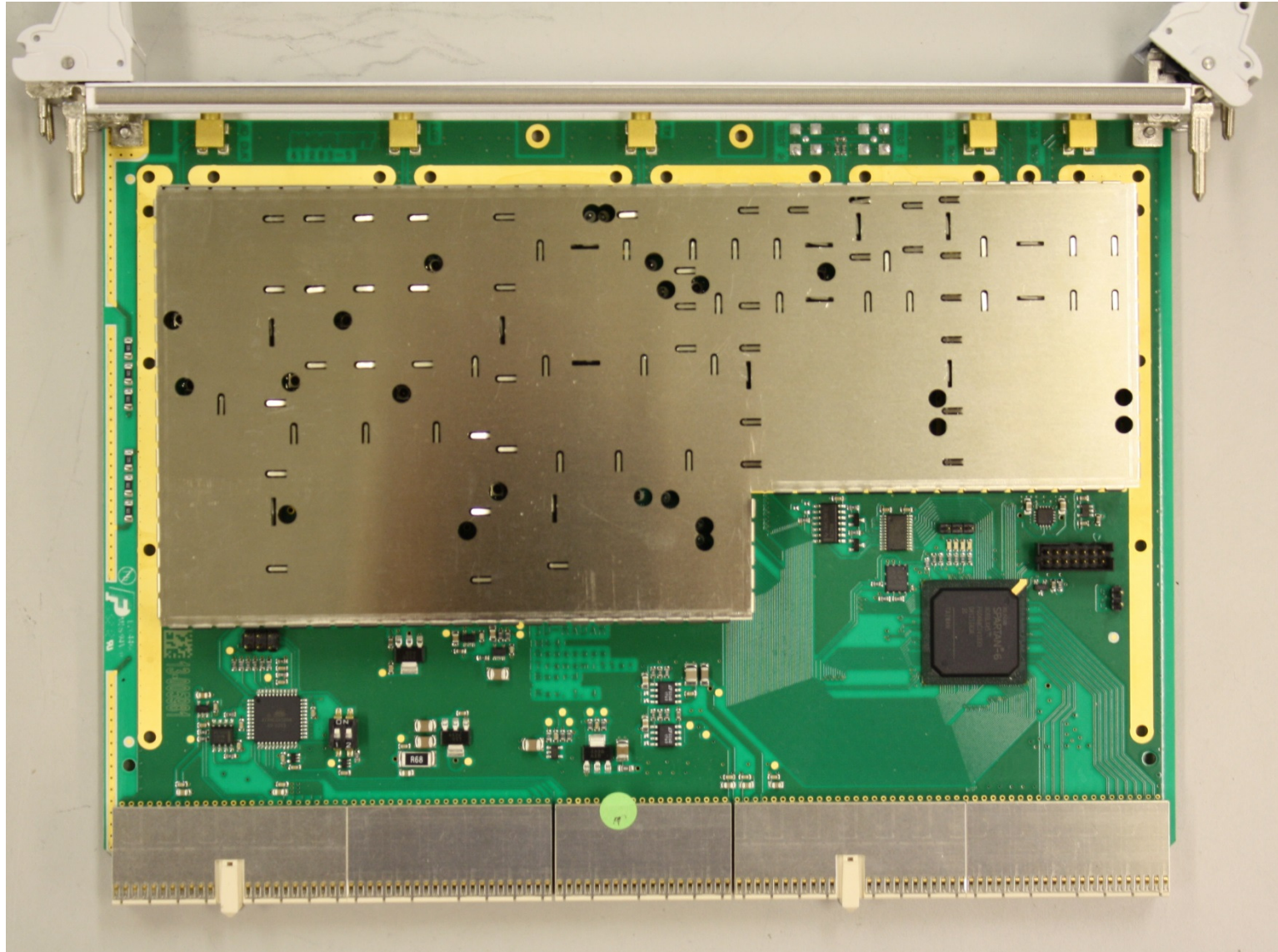
3d-Radar Geoscope Transmitter board. Top view. Shielded.
