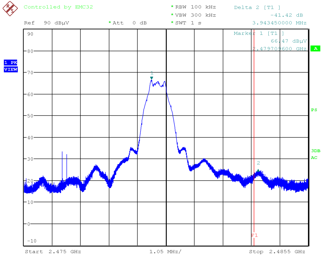
Band edge compliance of radiated emissions
