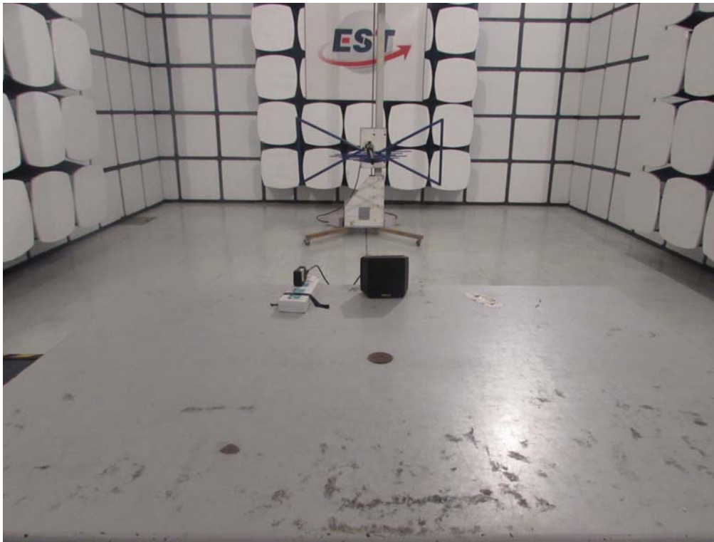
Radiated Test (30-1000 MHz) (Adapter 2)
