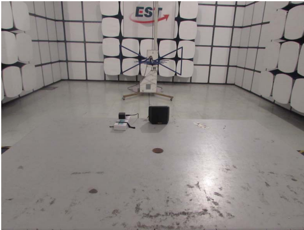
Radiated Test (30-1000 MHz) (Adapter 1)
