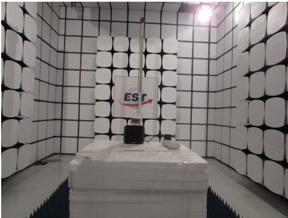
Radiated Test (1000-25000 MHz) (Adapter 1)
