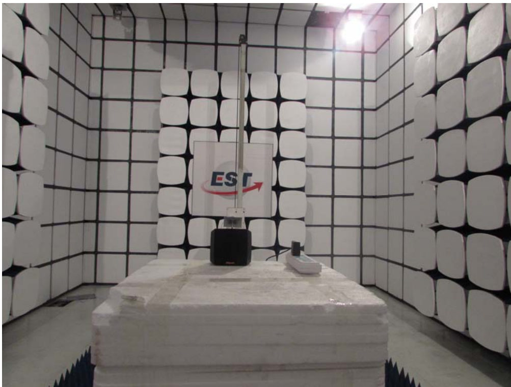
Radiated Test (1000-25000 MHz) (Adapter 2)
