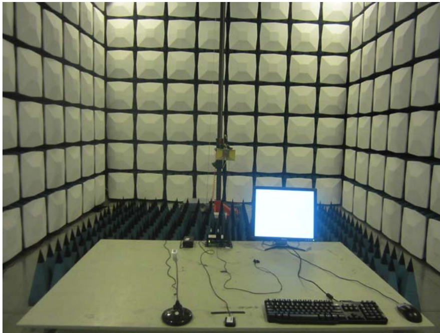
Radiated Emission – Front View (Above 1GHz Distance of 3m)
