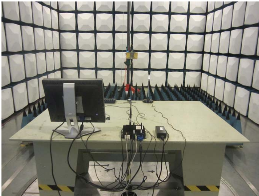
Radiated Emission – Rear View (Above 1GHz Distance of 3m)
