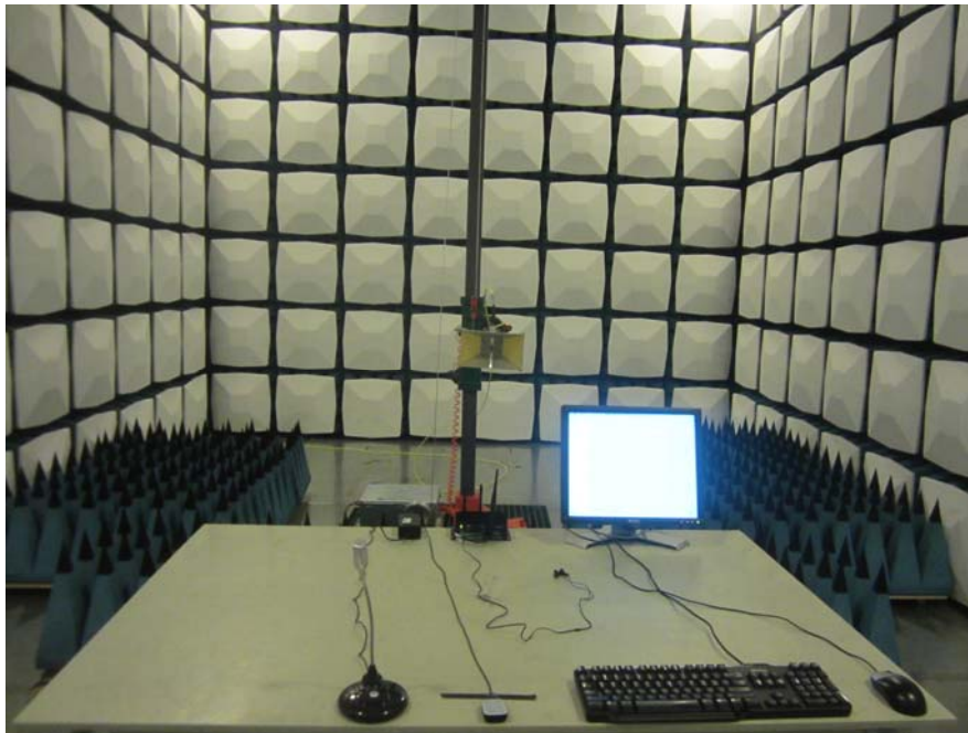
Radiated Emission – Front View (Above 1GHz Distance of 1.5m)
