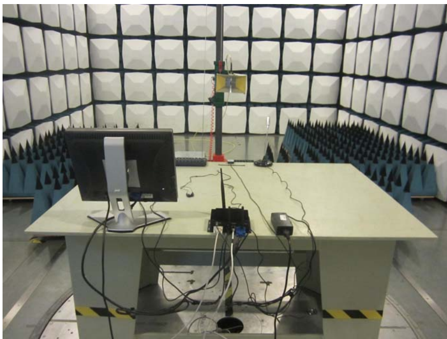
Radiated Emission – Rear View (Above 1GHz Distance of 1.5m)
