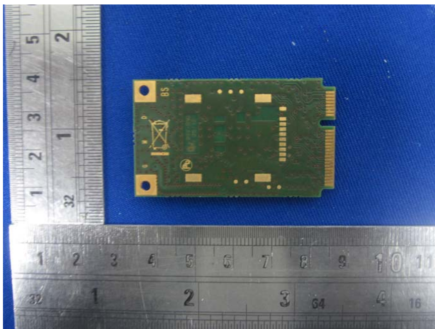
EUT –3G Module Bottom View
