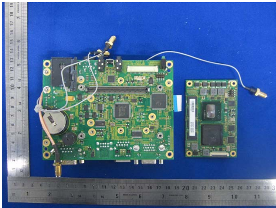
EUT – All Board Uncover 2 View
