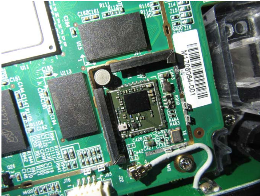
EUT_WLAN & Bluetooth RF Module Shielding off View
