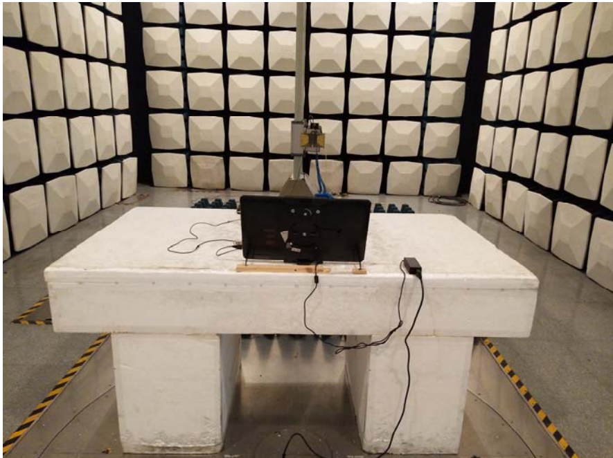
Radiated Disturbance Test Setup Rear View (Above 1GHz)
