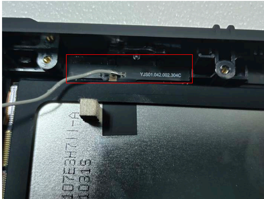
EUT – LTE Diversity Antenna 1 View
