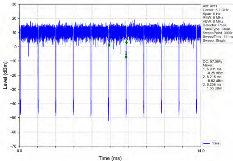
802.11ac(VHT20)_MCH_5200MHz_Ant1_NTNV
