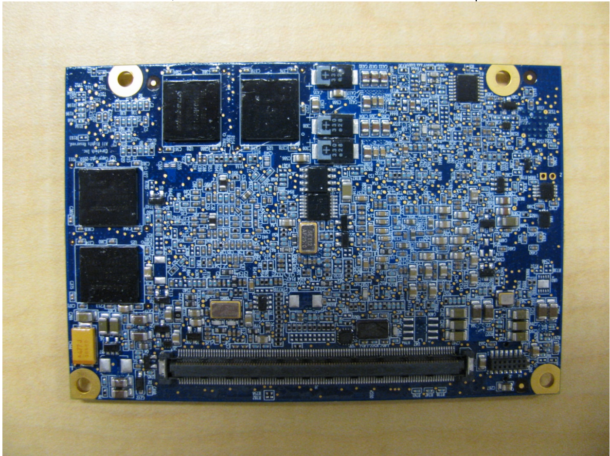
Circuit Board, 900125-5015R Rev J 1.6 GHz Intel Atom Module top view
