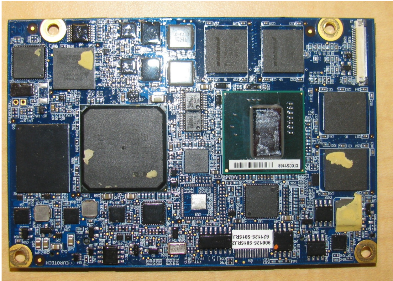
Circuit Board, 900125-5015R Rev J 1.6 GHz Intel Atom Module back view
