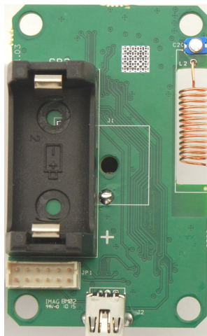
CT-151, CT-152, CT-154, CT-155, CT-156 - Rear View
