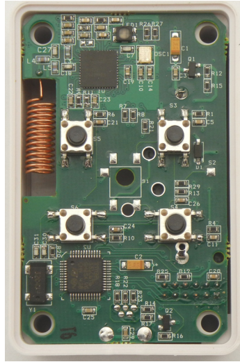
CT-152 & CT-154 - Front View
