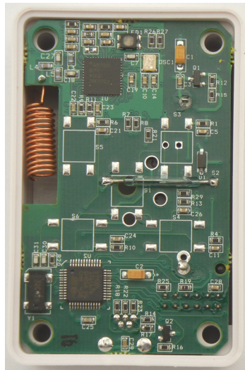
CT-155 - Front View
