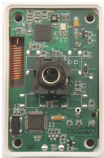
CT-156 - Front View
