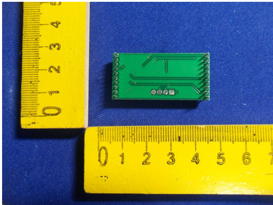
Figure 10 PCB of the EUT
