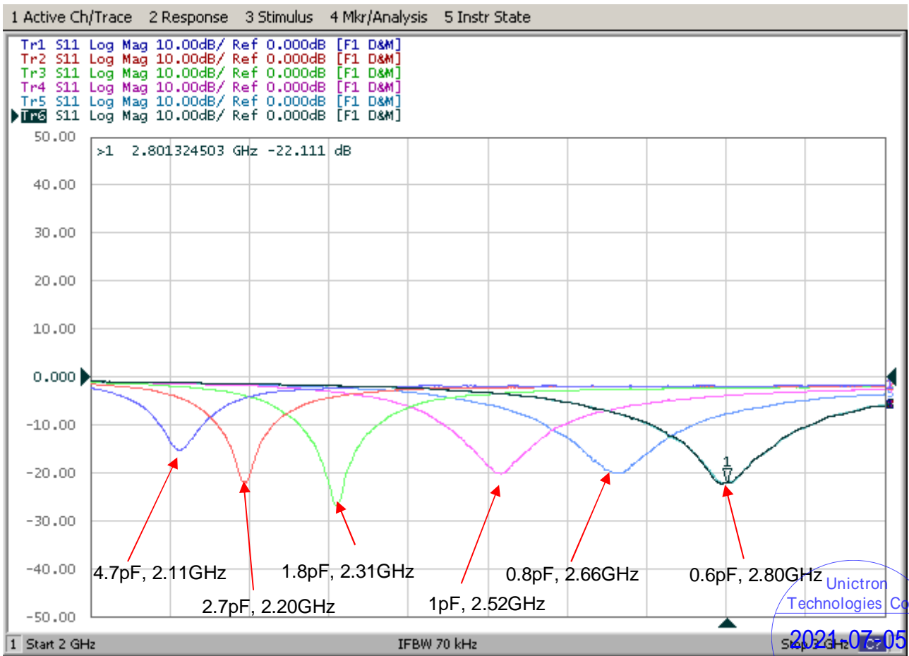
Frequencies vs. capacitance of tuning element
