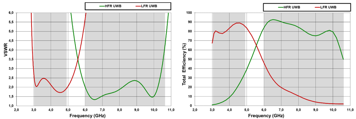
Figure 14 – VSWR and total efficiency for the UWB LFR (3.1GHz – 4.8GHz) and for the UWB HFR (6.0GHz – 10.6GHz) from the Evaluation Board ( Figure 11 with the matching networks gathered in Figure 12 (LFR UWB) and Figure 13 (HFR UWB), respectively. Simulated results obtained with CST.
