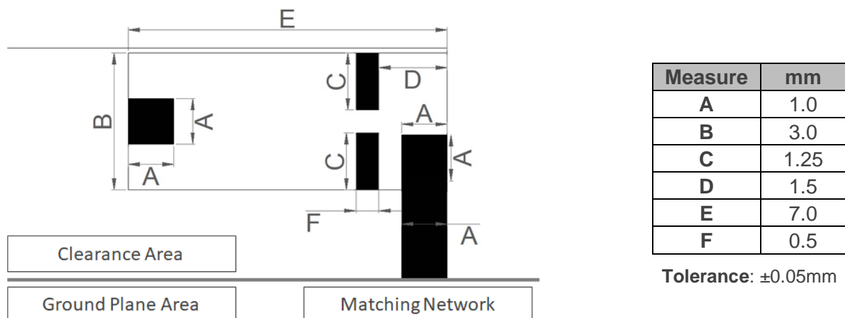
Figure 15 – Footprint dimensions for the NN03-320 in the corner for UWB.
