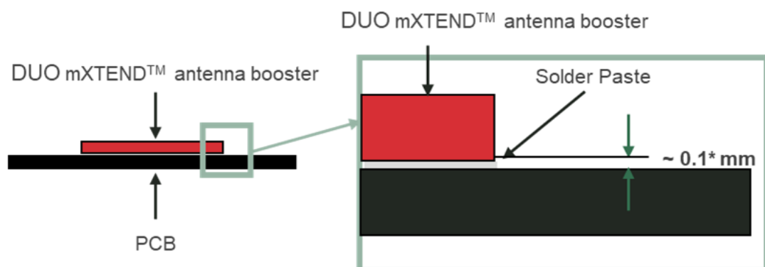
Figure 19 – Soldering Details.
