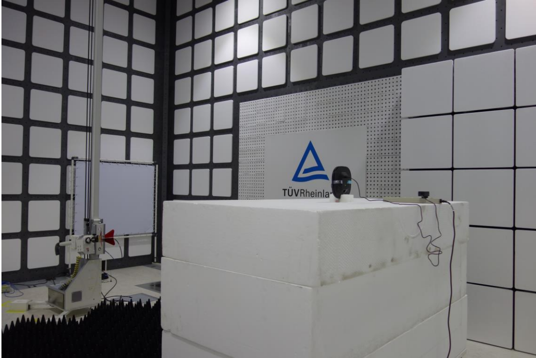
Photograph 5: Set-up for Spurious Emissions (Back View 3)
