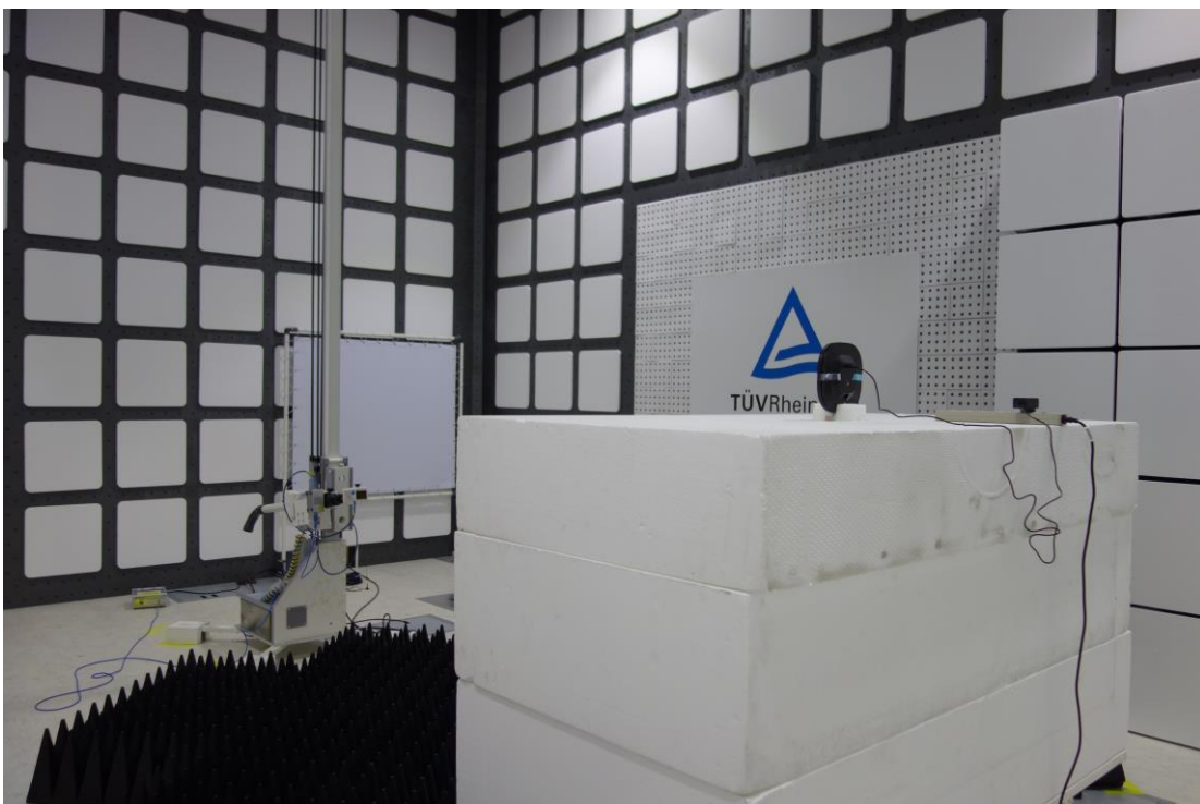
Photograph 6: Set-up for Spurious Emissions (Back View 4)
