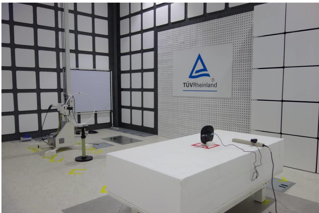
Photograph 4: Set-up for Spurious Emissions (Back View 2)
