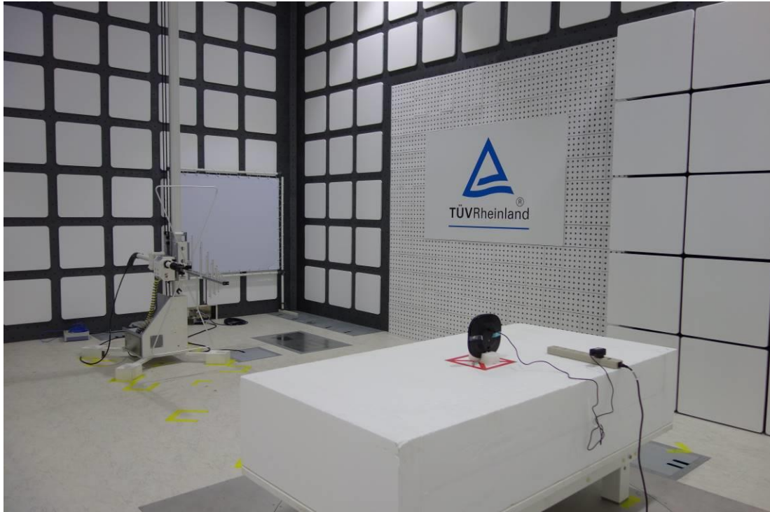
Photograph 3: Set-up for Spurious Emissions (Back View 1)
