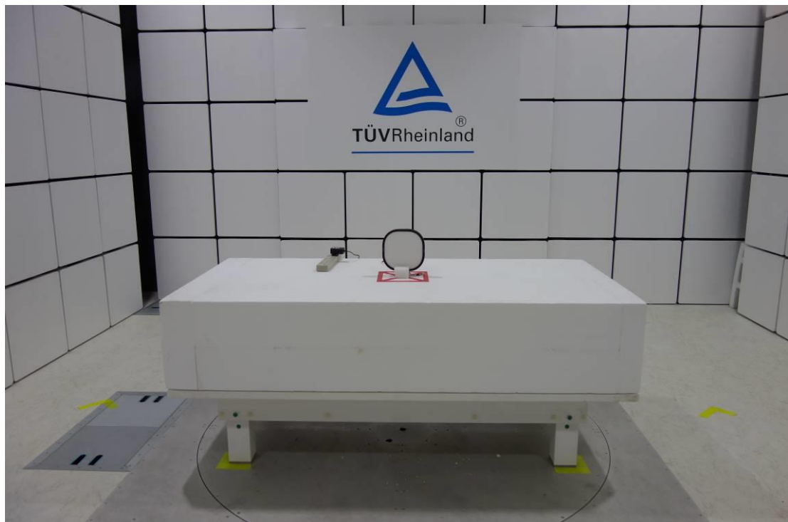
Photograph 2: Set-up for Spurious Emissions (Front View 2)
