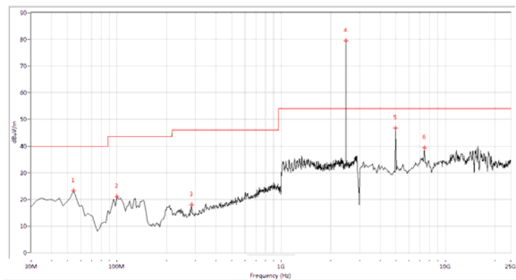
(30MHz to 25GHz, Antenna Horizontal @ \pi/4 -DQPSK, channel 78)
