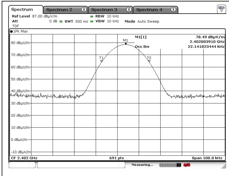
99% bandwidth
