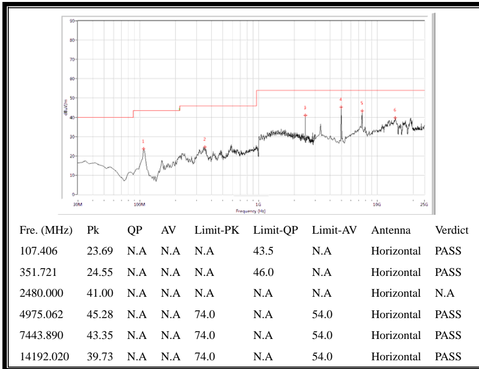
(30MHz to 25GHz, Antenna Horizontal @ \pi/4 -DQPSK, channel 78)
