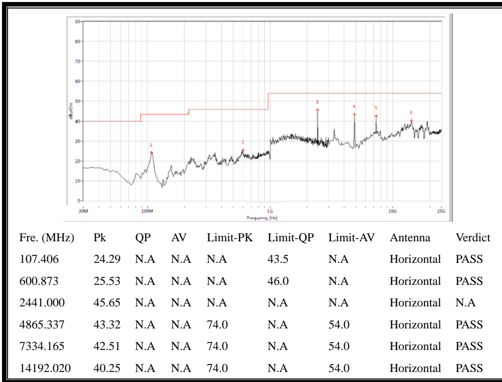
(30MHz to 25GHz, Antenna Horizontal @8-DPSK, channel 39)
