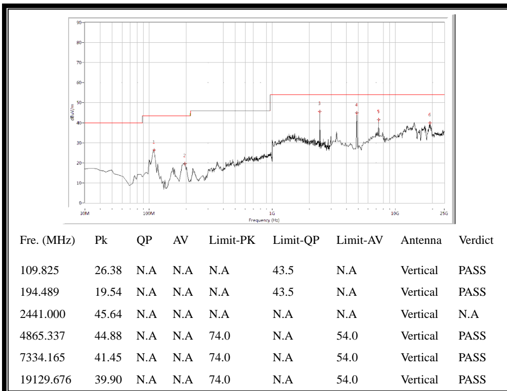
(30MHz to 25GHz, Antenna Vertical @ GFSK, channel 39)
