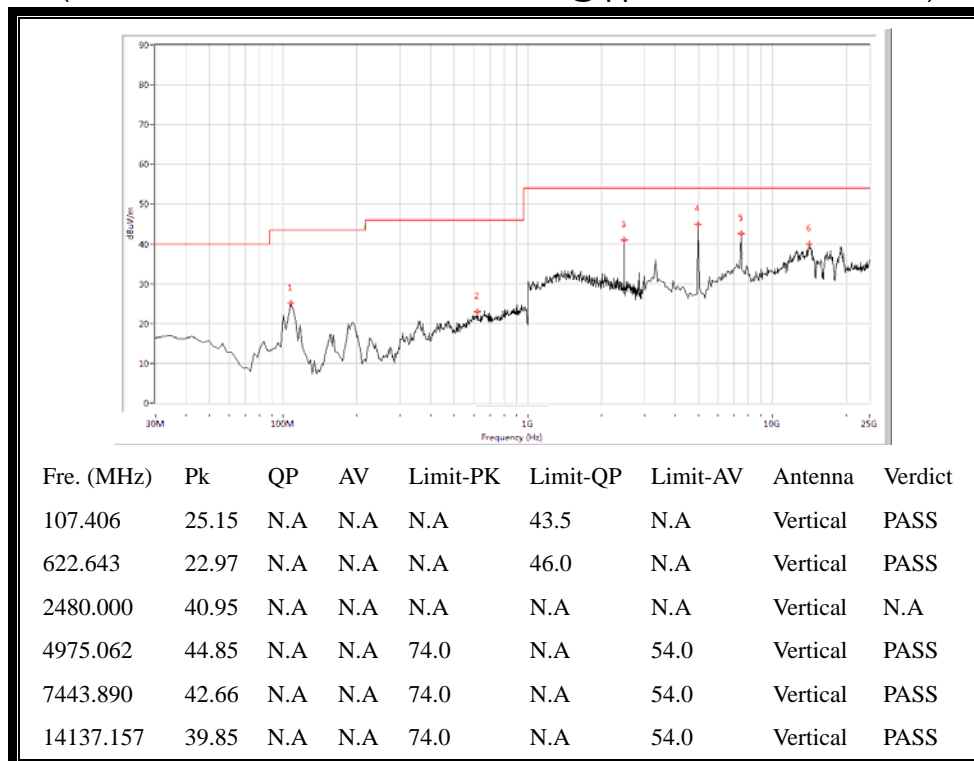
(30MHz to 25GHz, Antenna Vertical @ \pi/4 -DQPSK, channel 78)
