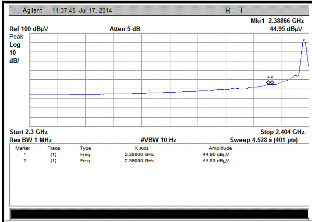
(Plot A2:Channel = 0 AVERAGE @ GFSK)
