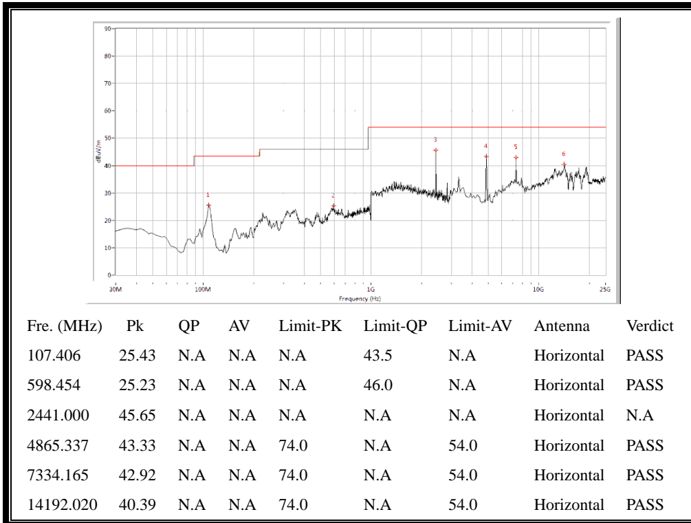
(30MHz to 25GHz, Antenna Horizontal @ GFSK, channel 39)
