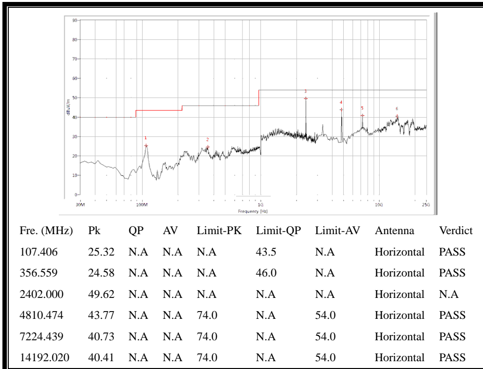
(30MHz to 25GHz, Antenna Horizontal @ GFSK, channel 0)
