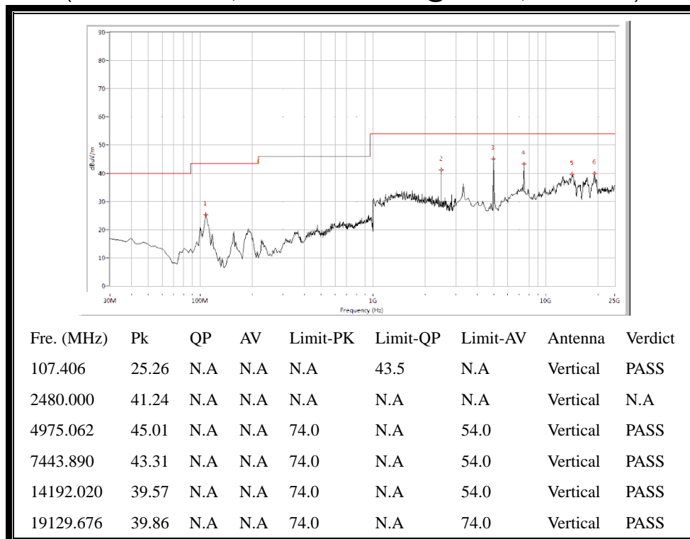
(30MHz to 25GHz, Antenna Vertical @8-DPSK, channel 78)
