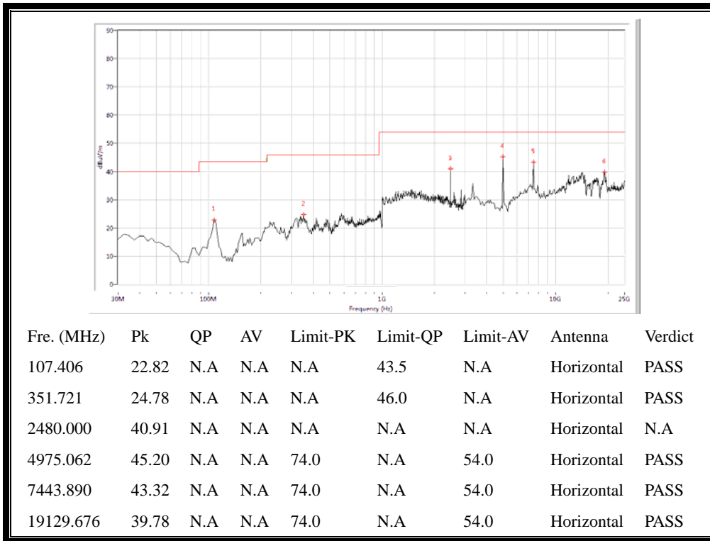
(30MHz to 25GHz, Antenna Horizontal @ GFSK, channel 78)
