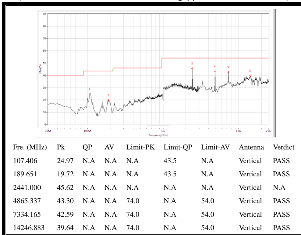
(30MHz to 25GHz, Antenna Vertical @ \pi/4 -DQPSK, channel 39)
