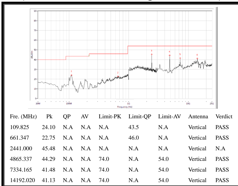
(30MHz to 25GHz, Antenna Vertical @8-DPSK, channel 39)
