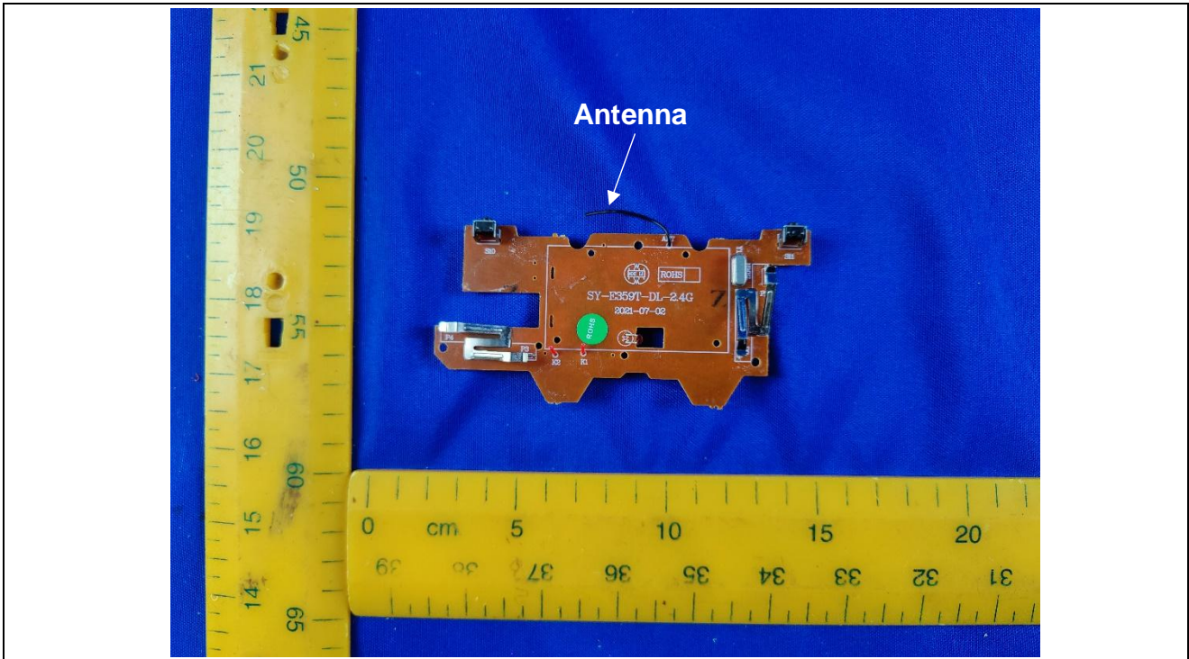
Details of: PCB view for remote controller
