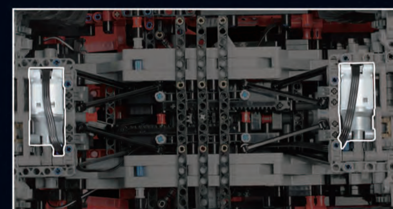
The front and rear axles are equipped with independent motors
