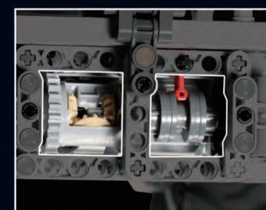
The front and rear axles are equipped with independent radio-control differential lock
