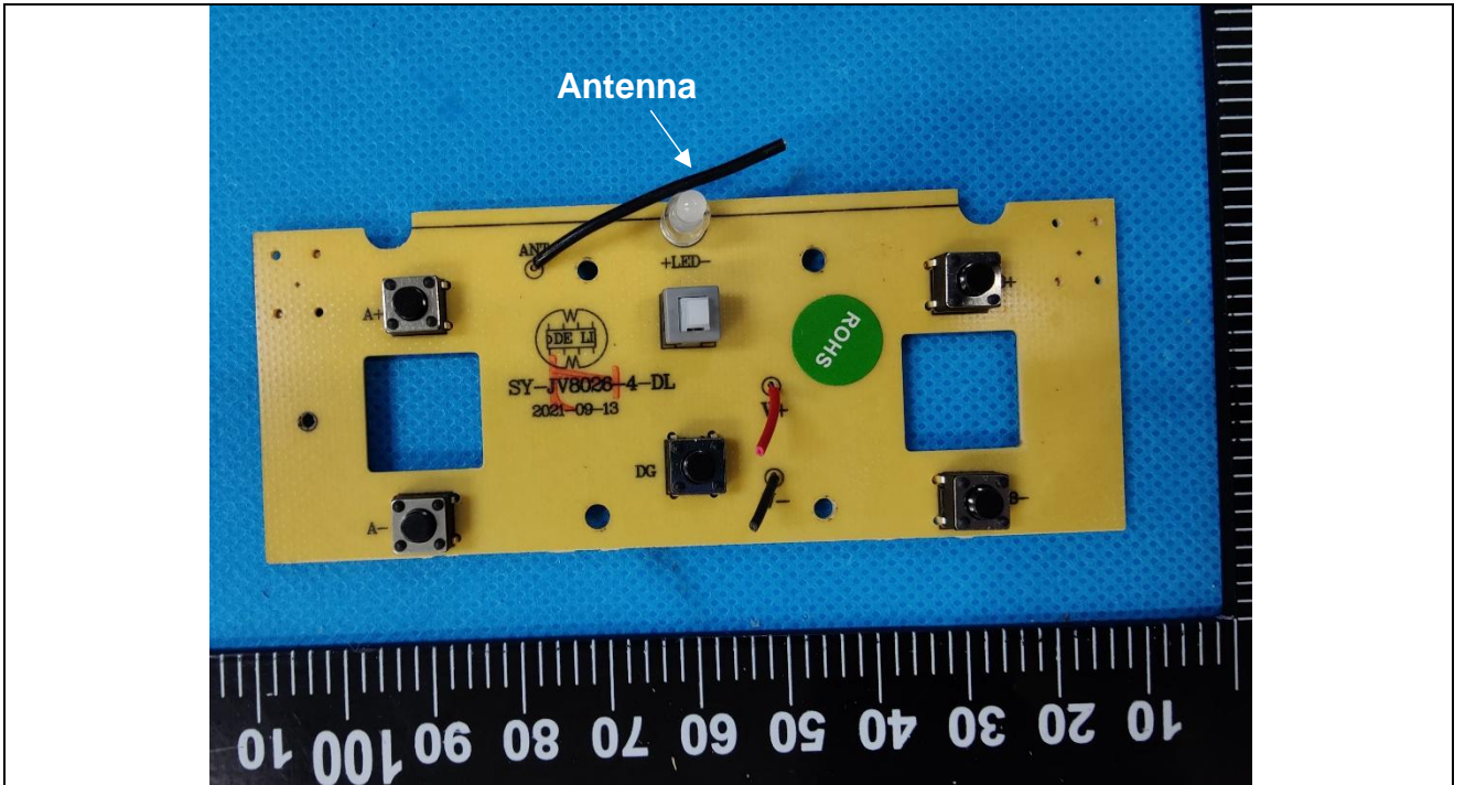
Details of: PCB view for Remote controller
