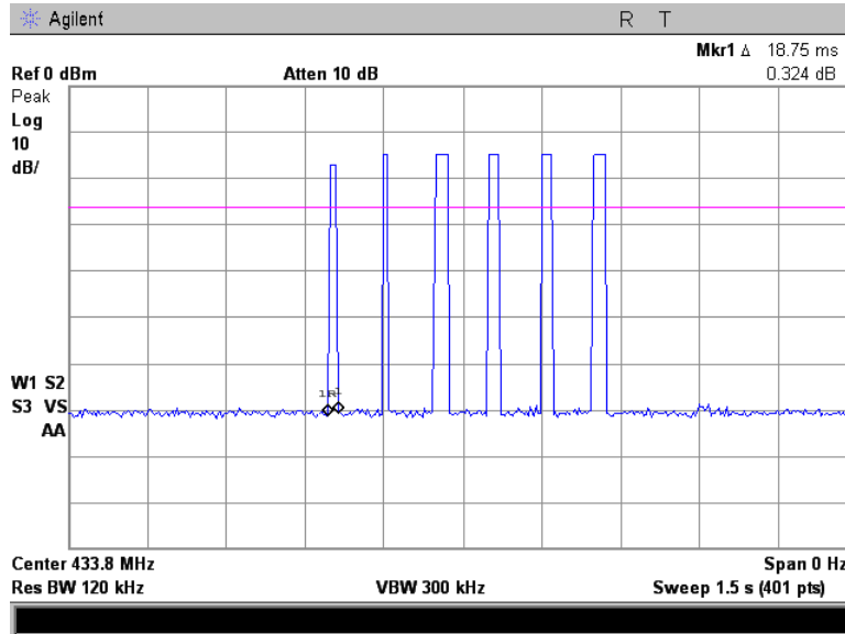
Plot 7.2.24 Transmitter pulse duration
