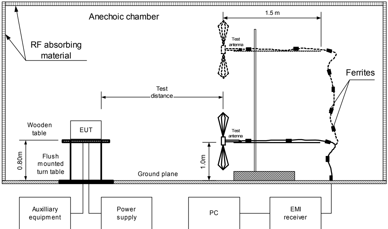
Figure 8.2.1 Setup for radiated emission measurements in anechoic chamber, table-top EUT
