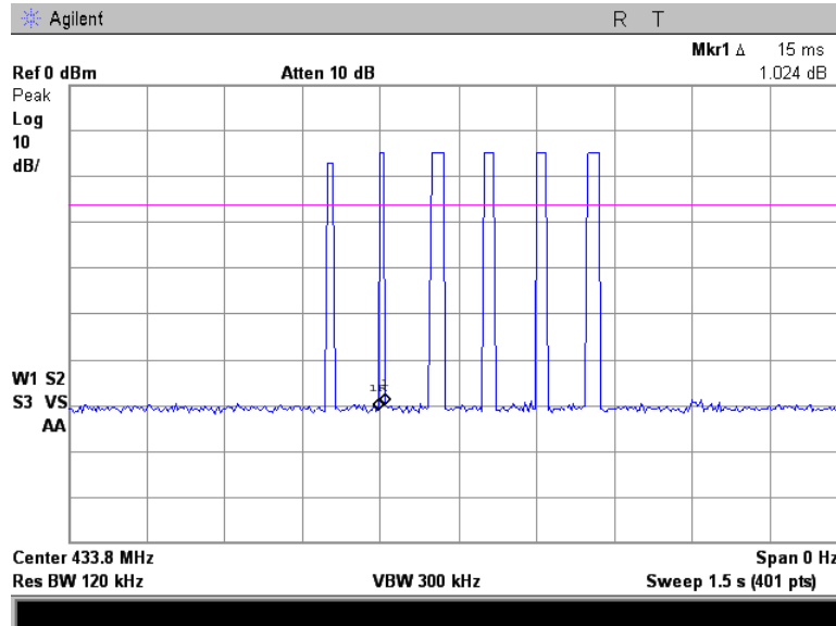
Plot 7.1.3 Transmitter pulse duration
