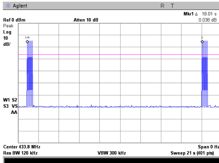
Plot 7.2.28 Transmission burst period
