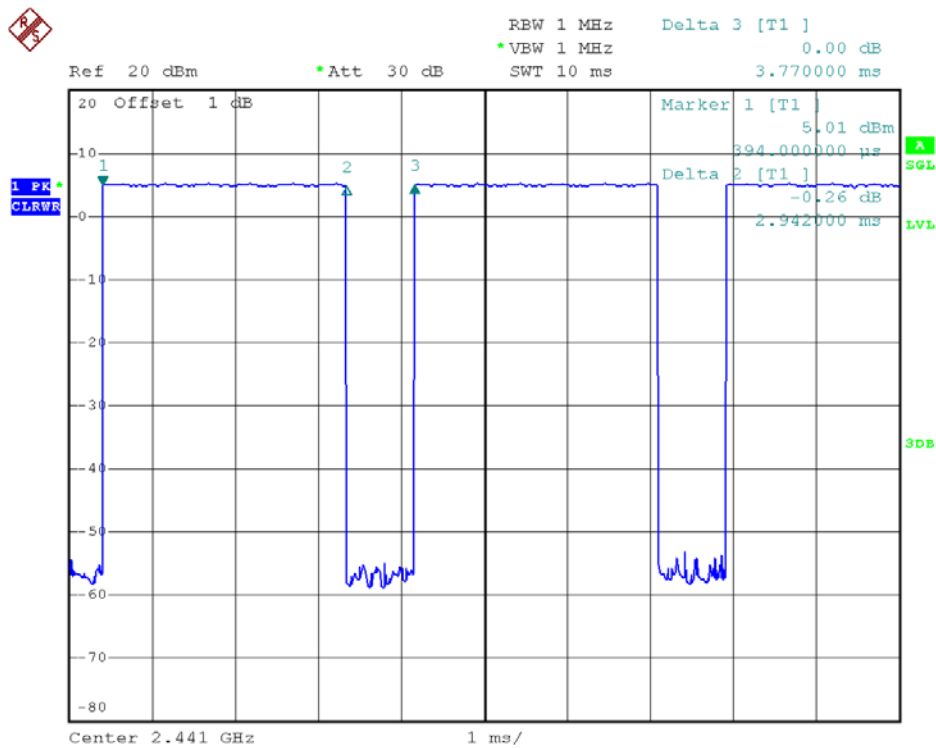
39 Channel @ 2DH5
