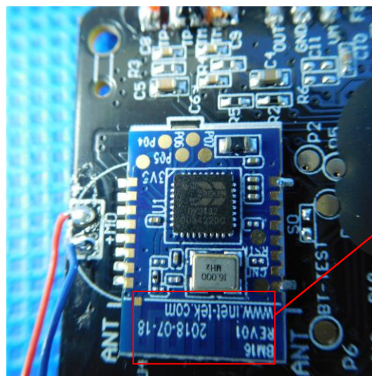
BT Antenna
