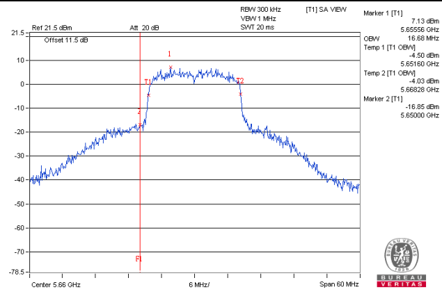
802.11a / Chain 1 – CH132
