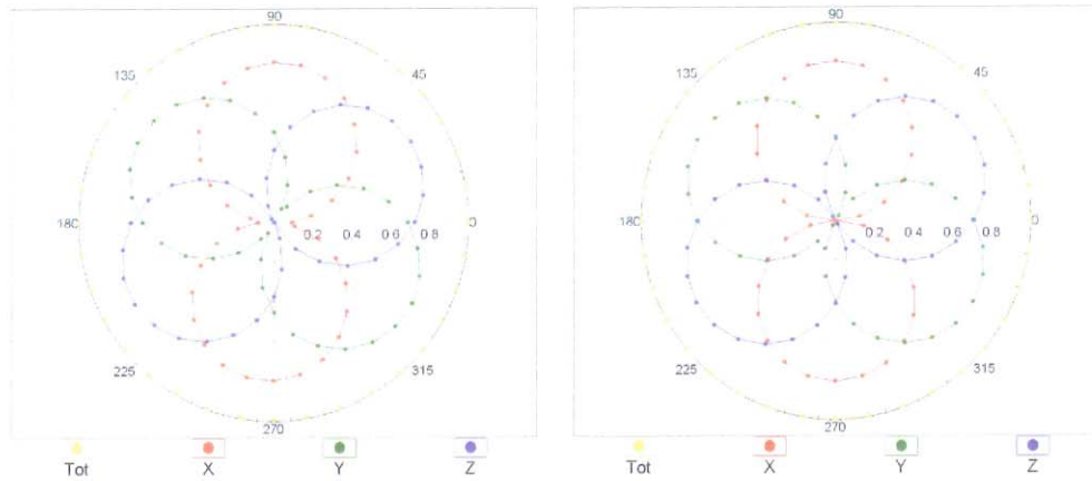
f=600 MHz,TEM
