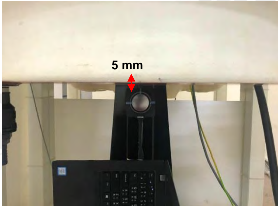
Fig.9 EUT Top side to flat phantom
