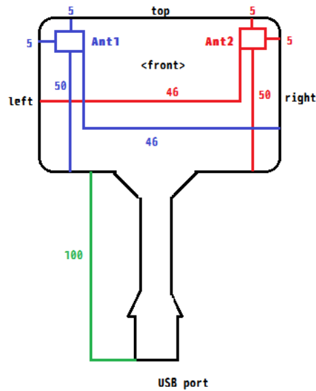
Fig.17 Antenna location of EUT
