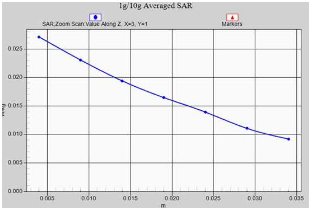
GSM850 LEFT/CHEEK-Low_ z-axis scan
