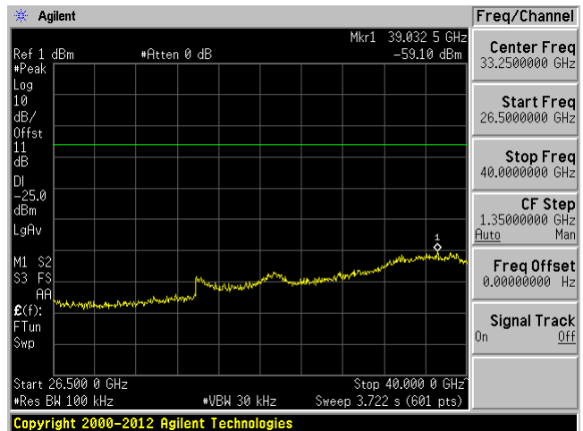
Low Channel 5875 MHz Chain 1, 26.5GHz – 40GHz
