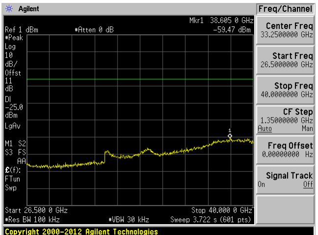
Low Channel 5875 MHz Chain 3, 26.5GHz – 40GHz
