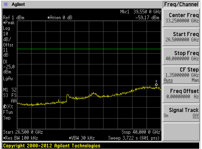
Low Channel 5875 MHz Chain 2, 26.5GHz – 40GHz
