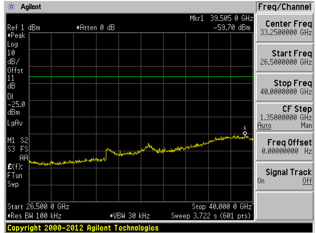
Low Channel 5875 MHz Chain 0, 26.5GHz – 40GHz
