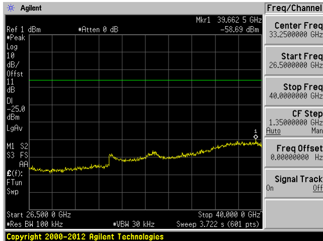
Low Channel 5875 MHz Chain 0, 26.5GHz – 40GHz
