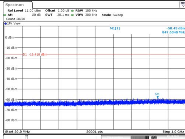
BLE_1M_Ant1_2402_30~1000
