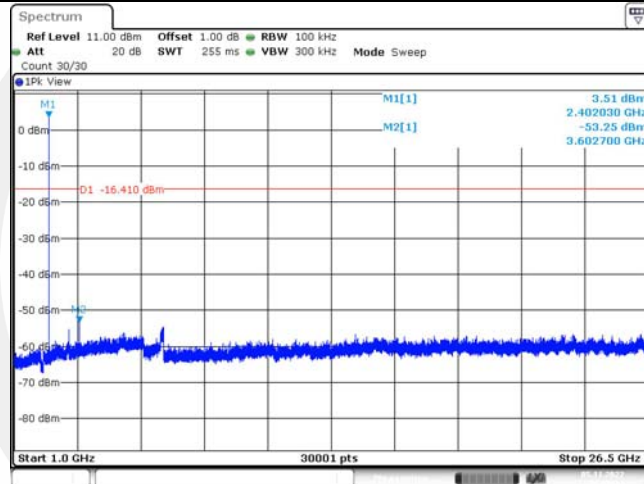
BLE_1M_Ant1_2402_1000~26500
