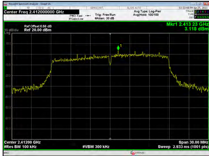
Tx. Spurious NVHT n20 2412MHz Ant1 Emission
