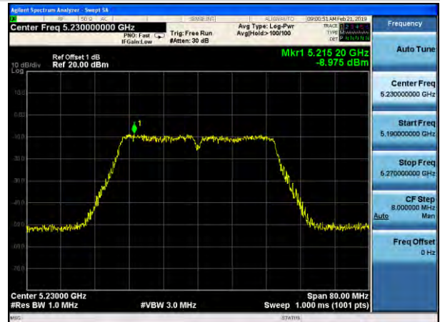
Channel 46 (5230MHz)
