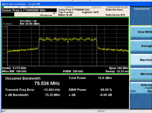
Channel 155(5775MHz)
