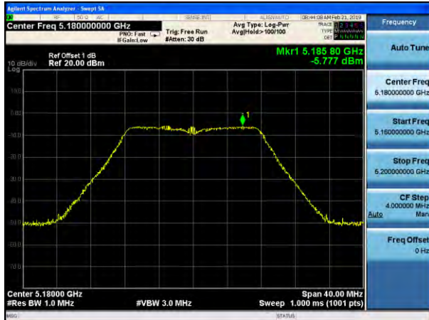
Channel 36 (5180MHz)
