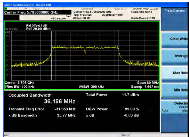
Channel 159 (5795MHz)
