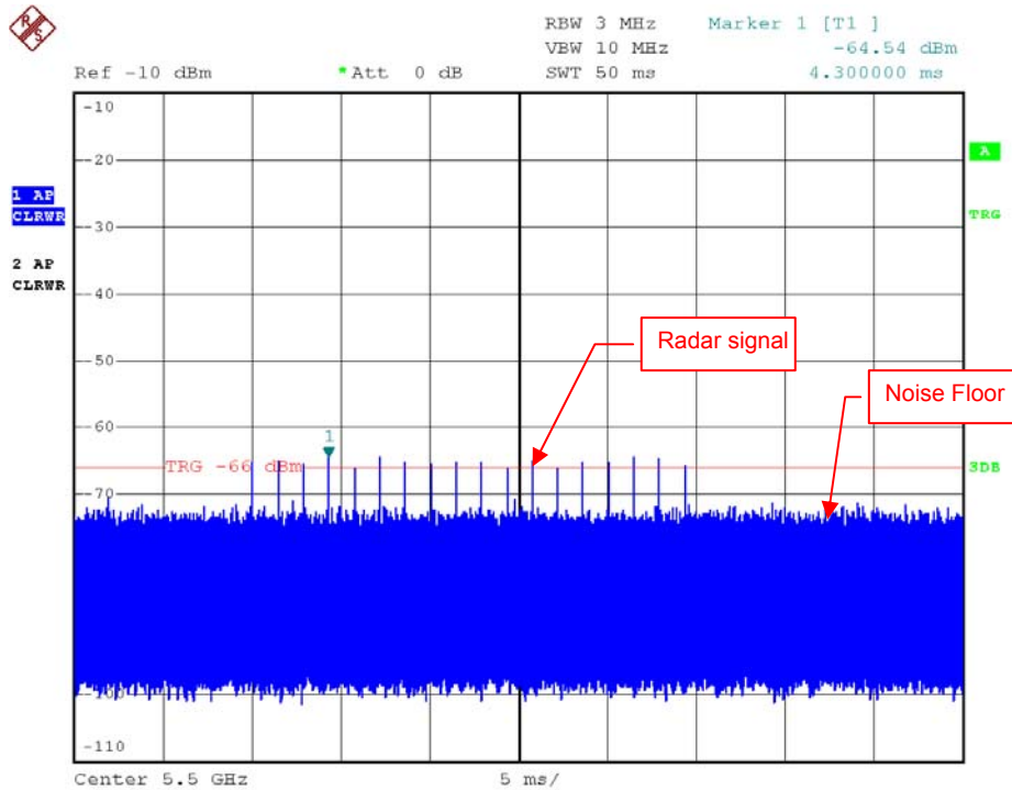
Radar Signal 0
