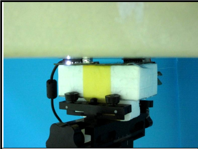
Front Face of EUT with 0.4 cm Gap
