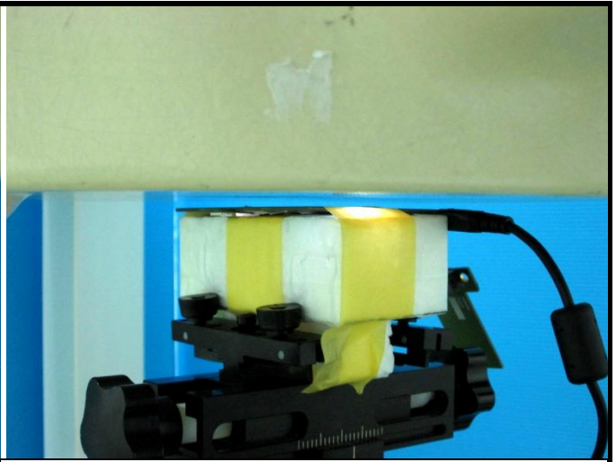
Rear Face of EUT with 0.4 cm Gap
