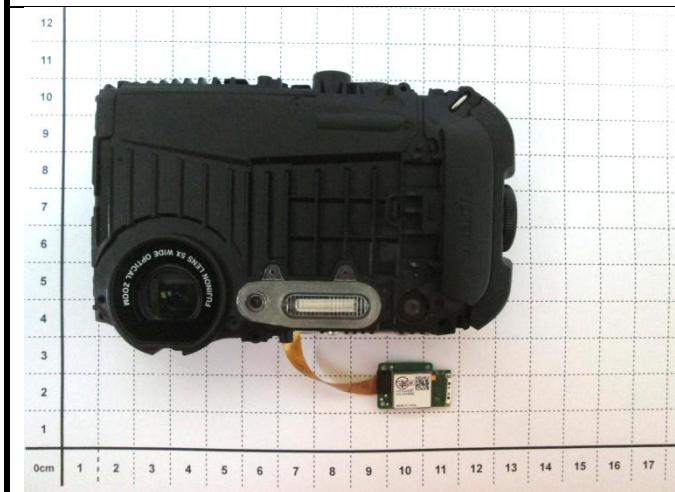
EUT Host – Front View
