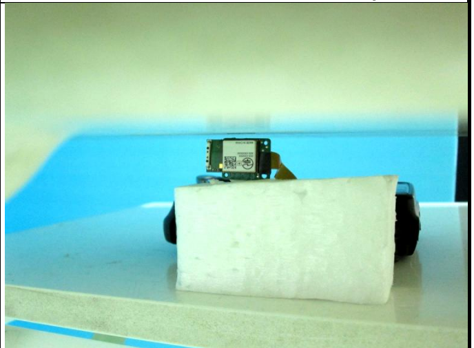
Right Side of EUT with 0.2 cm Gap
