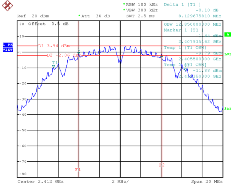
IEEE 802.11b/2412 MHz/6 dB and 99% Occupied Bandwidth
