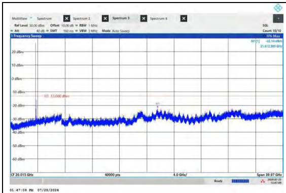
NTNV-N77-3700-3980-PC3-30-100-L-CP-QPSK-Edge_1RB_Left-Ant4-PASS
