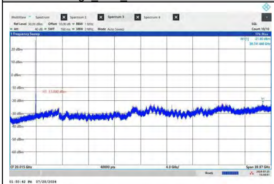
NTNV-N77-3700-3980-PC3-30-100-H-CP-QPSK-Edge_1RB_Left-Ant4-PASS
