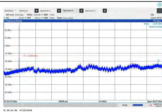
NTNV-N77-3700-3980-PC3-30-100-M-CP-QPSK-Edge_1RB_Left-Ant4-PASS
