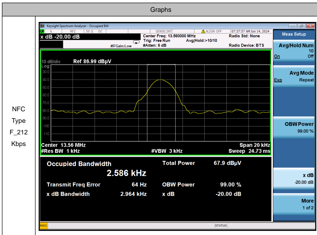
20dB Bandwidth & 99% Bandwidth Plot
