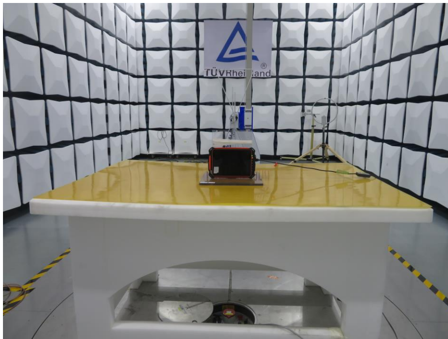
Photograph 3: Set-up for Radiated Emission, Up to 1GHz
