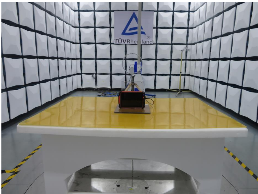
Photograph 2: Set-up photo for Radiated Emission, Below 30MHz
