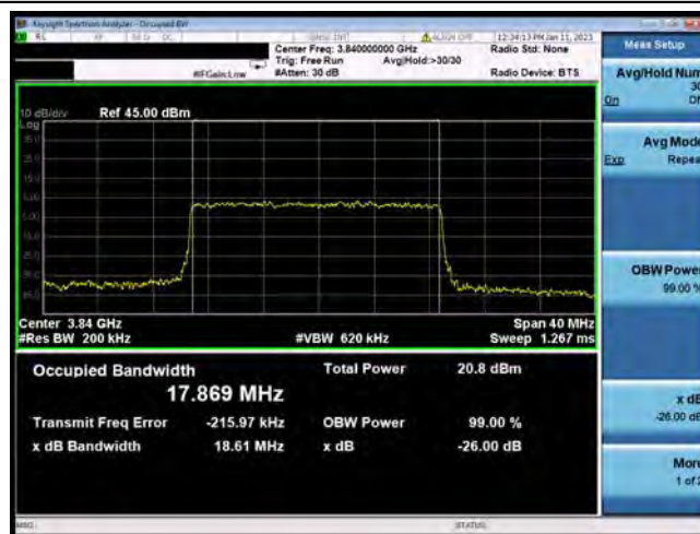
N77-20MHz-256QAM-656000-50RB#0
