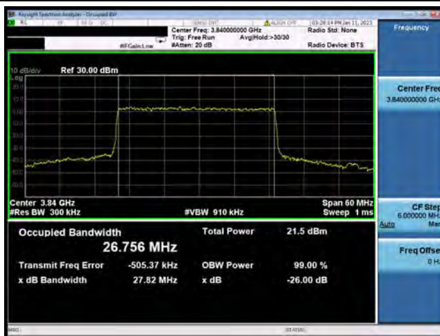
N77-30MHz-256QAM-656000-75RB#0
