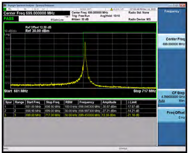
N12-15MHz-QPSK-141300-75RB#0
