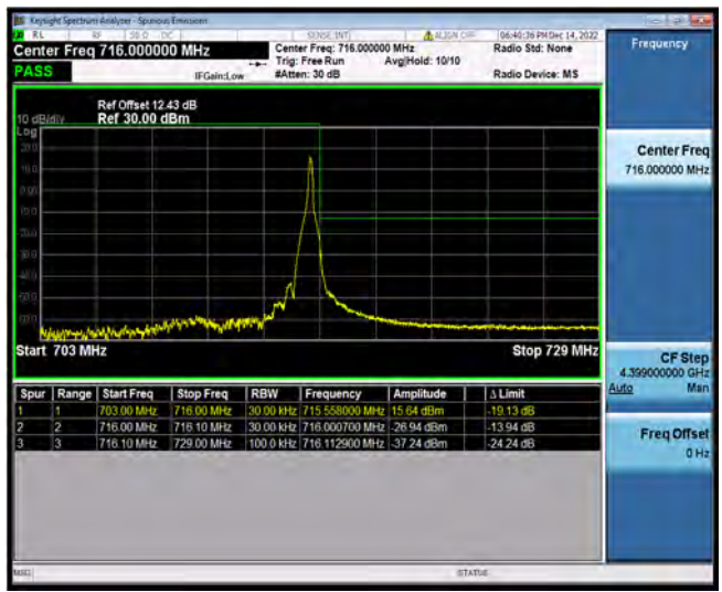
N12-10MHz-QPSK-142200-50RB#0
