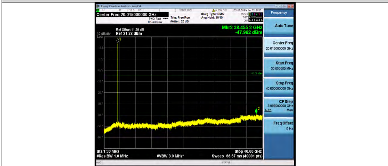
42-42-20MHz-20MHz-16QAM-16QAM-42792-42990-1RB#99-1RB#0-30~40000MHz
