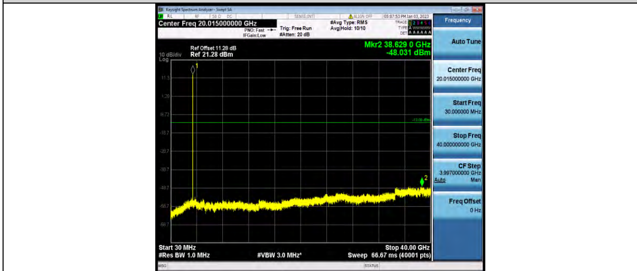
42-42-20MHz-20MHz-64QAM-64QAM-42491-42689-1RB#99-1RB#0-30~40000MHz
