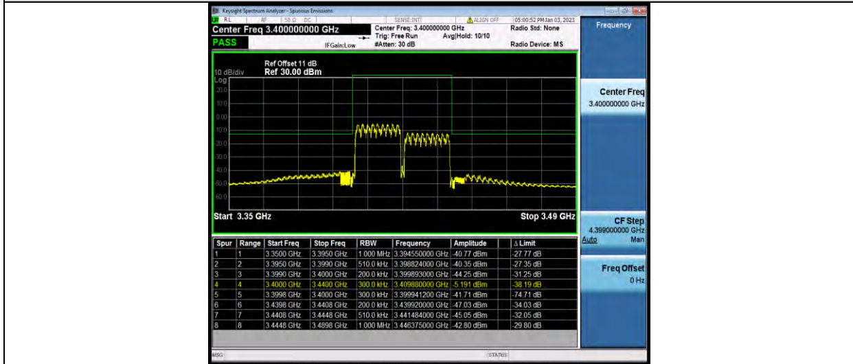
42-42-20MHz-20MHz-64QAM-64QAM-41690-41888-1RB#0-1RB#99
