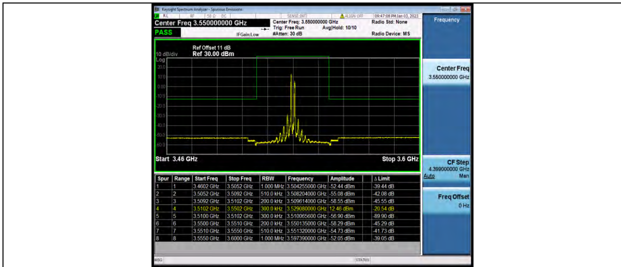
42-42-20MHz-20MHz-64QAM-64QAM-41690-41888-100RB#0-100RB#0
