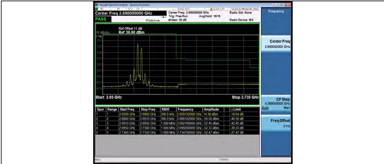
41-41-20MHz-20MHz-64QAM-64QAM-39750-39948-100RB#0-100RB#0
