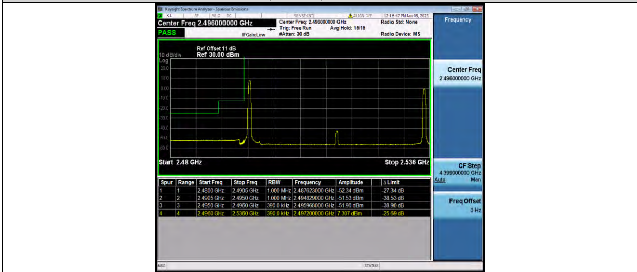
41-41-20MHz-20MHz-64QAM-64QAM-39750-39948-1RB#99-1RB#0
