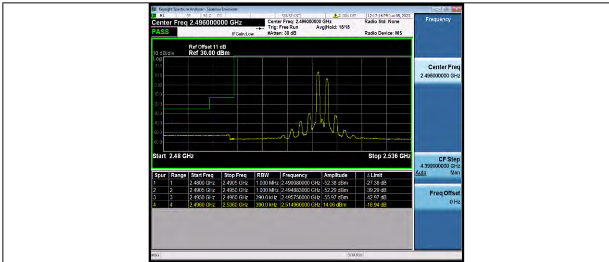
41-41-20MHz-20MHz-QPSK-QPSK-41292-41490-100RB#0-100RB#0
