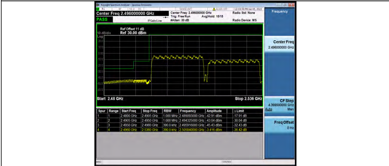
41-41-20MHz-20MHz-64QAM-64QAM-39750-39948-1RB#0-1RB#99
