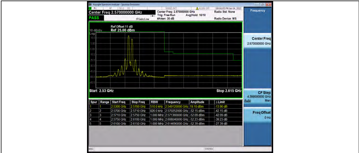
7-7-20MHz-20MHz-16QAM-16QAM-20850-21048-100RB#0-100RB#0
