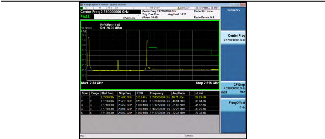
7-7-20MHz-20MHz-QPSK-QPSK-21152-21350-1RB#99-1RB#0
