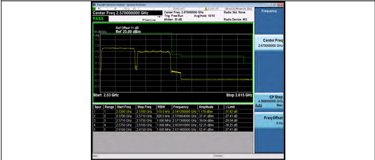
7-7-20MHz-20MHz-QPSK-QPSK-21152-21350-1RB#0-1RB#99
