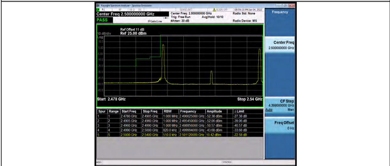
7-7-20MHz-20MHz-64QAM-64QAM-20850-21048-1RB#99-1RB#0
