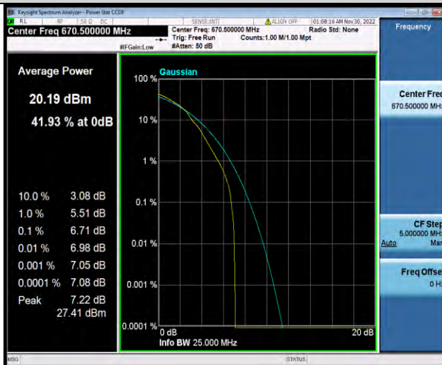
Band71-15MHz-64QAM-133197-75RB#0
