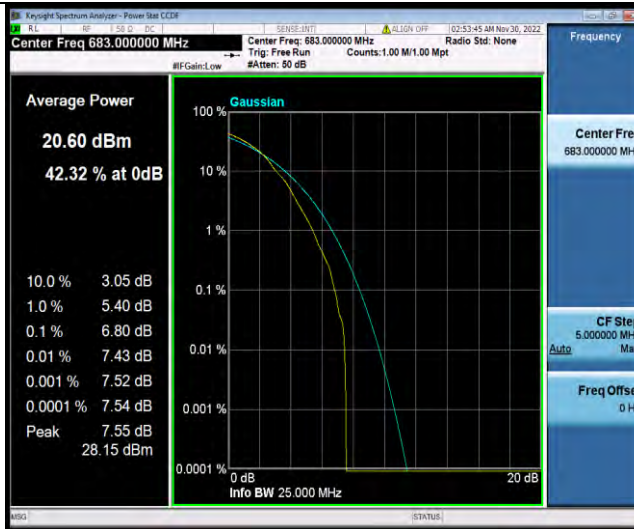
Band71-20MHz-64QAM-133322-100RB#0
