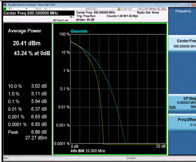
Band71-15MHz-64QAM-133197-1RB#0
