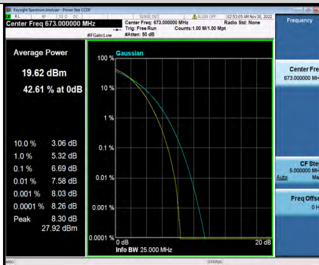
Band71-20MHz-64QAM-133322-1RB#0
