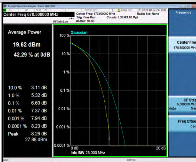
Band71-15MHz-64QAM-133297-1RB#0
