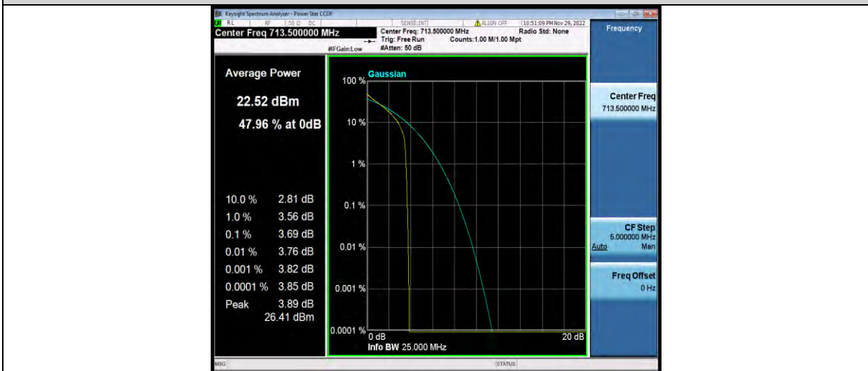
Band12-5MHz-QPSK-23155-25RB#0
