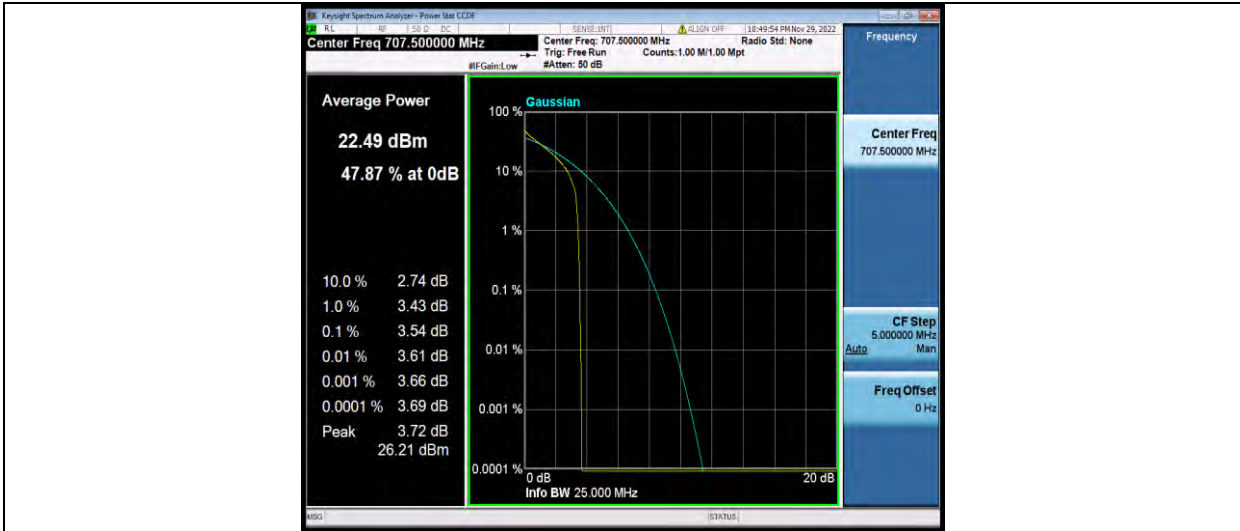
Band12-5MHz-QPSK-23095-25RB#0
