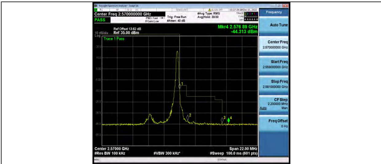
Band7-5MHz-QPSK-21425-25RB#0
