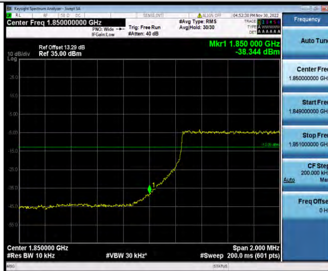
Band25-5MHz-QPSK-26065-1RB#24
